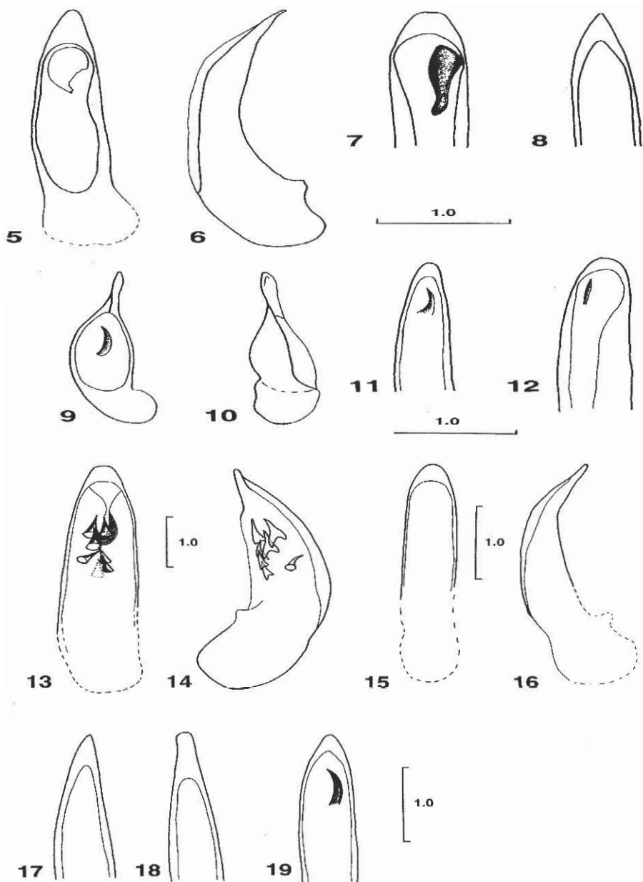
Figures 5-19. Median lobe of aedeagus. Figs. 5, 6. N. pseudolimbipennis , dorsal and lateral aspect, Fig. 7. N. disparilis dorsal aspect, Fig. 8. N. nebrioides , dorsal aspect, Figs. 9, 10. N. umbrifera , dorsal and lateral aspect, Fig. 11. N. flavicinctus , dorsal aspect, Fig. 12. N. viridula , dorsal aspect, Figs. 13, 14. N. maxima , dorsal and lateral aspect, Figs. 15, 16. N. glabrata , dorsal and lateral aspect, Fig. 17. N. aulica , dorsal aspect, Fig. 18. N. wilkensi , dorsal aspect, Fig. 19. N. jucunda , dorsal aspect (scales 1 mm, only Figs. 13, 14 smaller scale).
